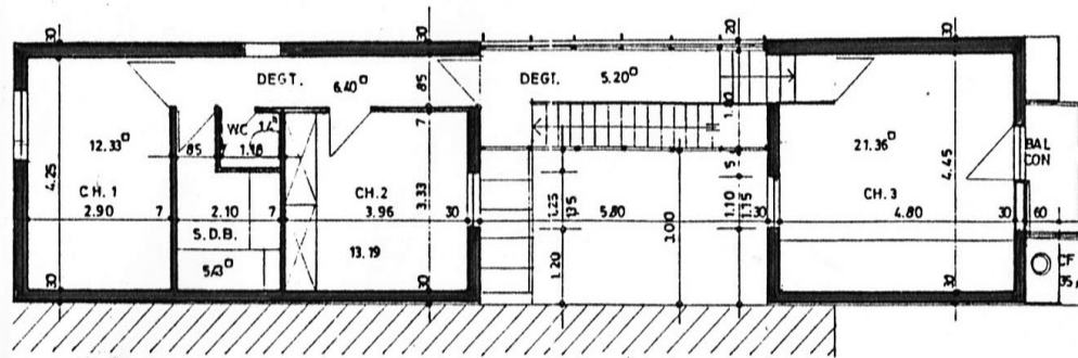
ETAGE 65.31m²
